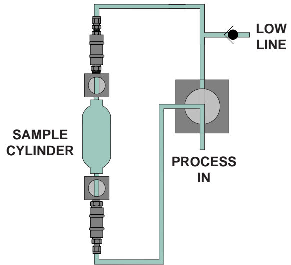
SEQUENCE 2 — Valve Position 2
