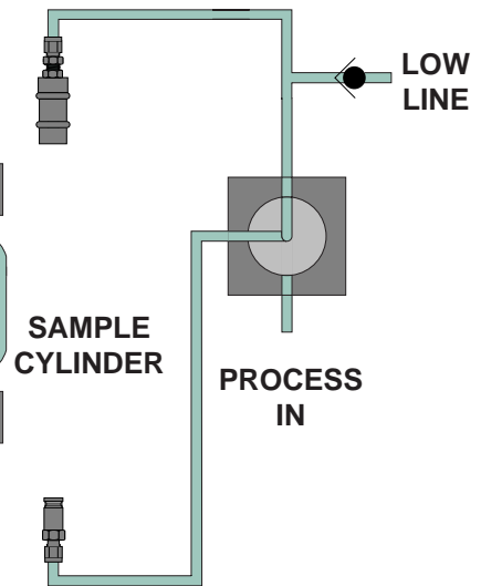
SEQUENCE 4 — Valve Position 1
